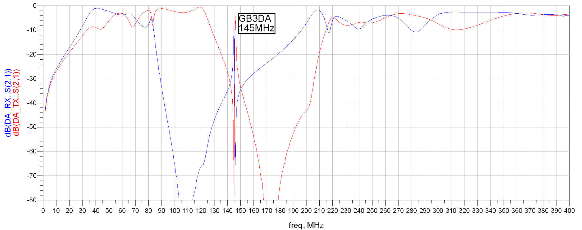
GB3DA Cavities Wide Band Plot - Nov 1996
