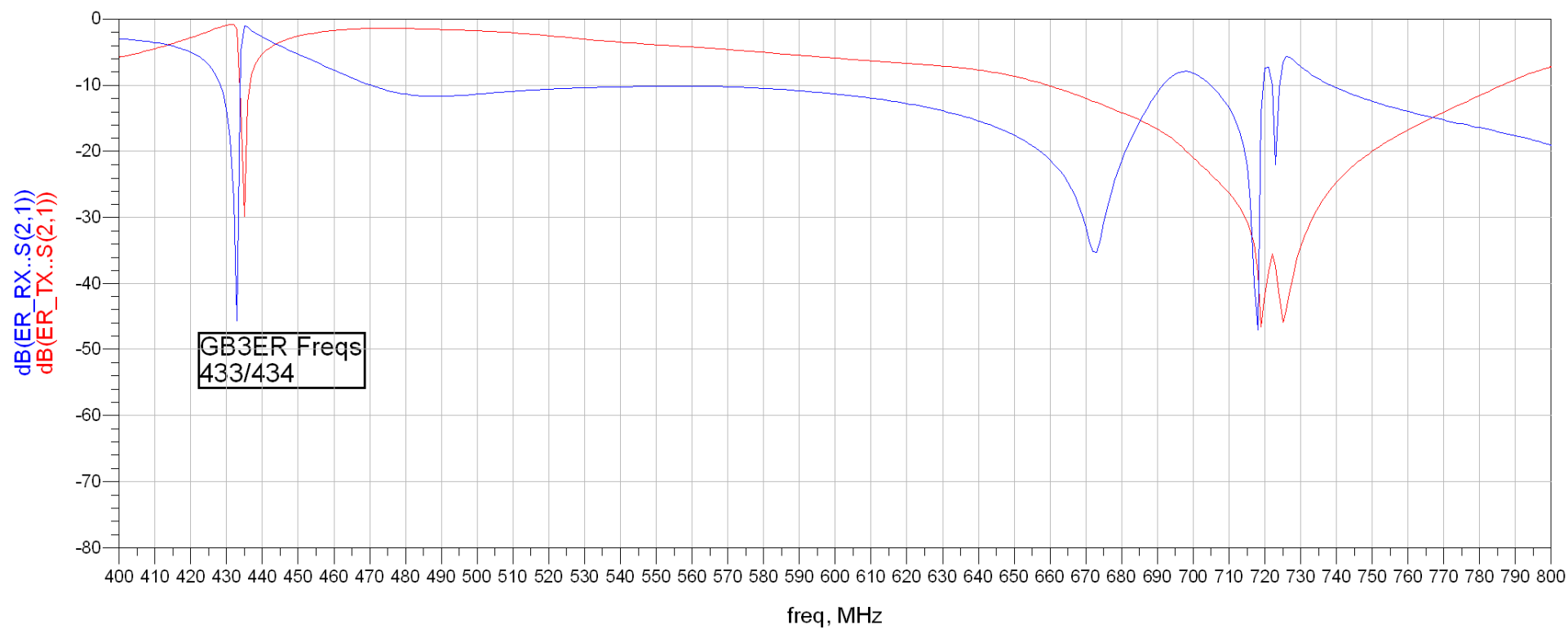
GB3ER Cavities Wide Band Plot - Nov 1996
