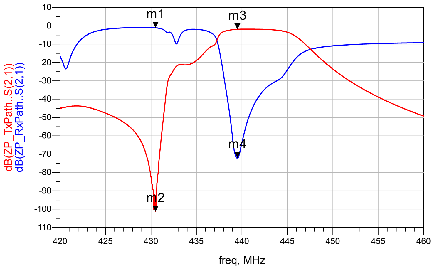
GB7ZP Duplexer - Tx and Rx Path Loss/Isolation
